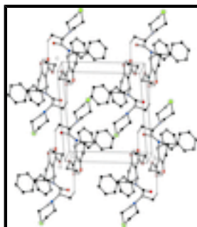
Fig. 2. The molecular packing of (I). For clarity, hydrogen atoms which are not involved in hydrogen bonding are omitted.
