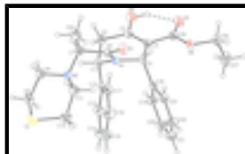
Fig. 1. The molecular structure of title compound, showing 30% probability displacement ellipsoids.
